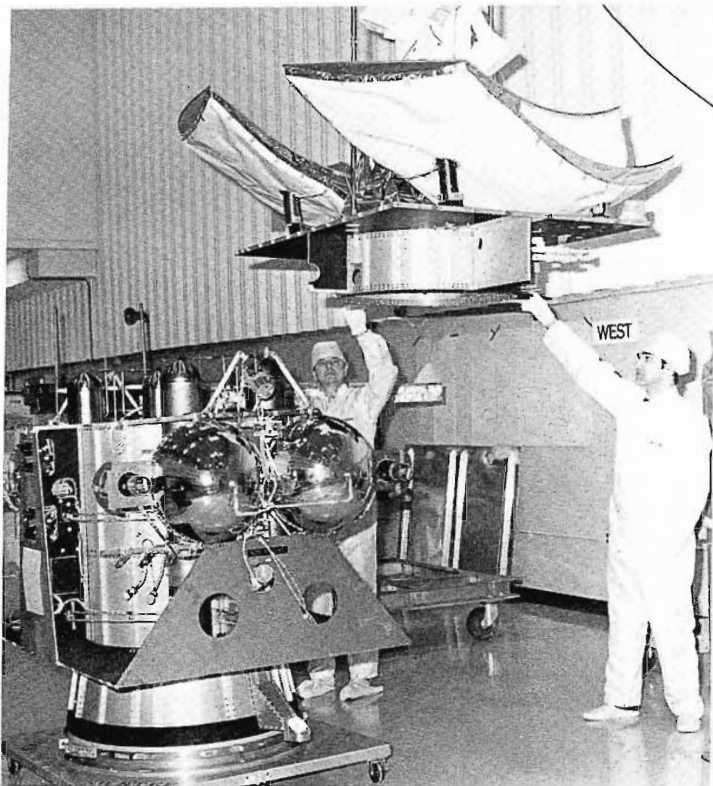
SATCOM III SATELLITE GETS ITS "TOP HAT" Engineers lower feed-horns and antennas to the RCA Satcom III-R commercial communications satellite. The C-band array will provide complete coverage of the contiguous states and Alaska, as well as a spot beam to Hawaii. The satellite is being assembled at RCA Astro-Electronics, Princeton, N. J., for RCA American Communications, also in Princeton.
