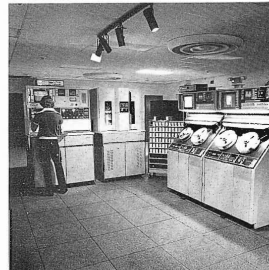
TR-600 quad VTR's are used for production and program playback; the video cartridge tape machine for airing commercials.
