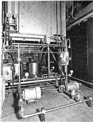
Ceiling-mounted diplexer (left) and heat exchanger (right) are designed for 110 kW operation.
