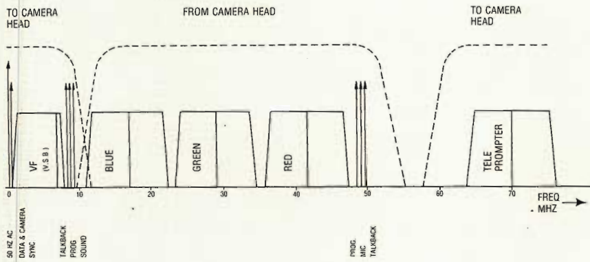
Fig. 6. TK-47 Triax Frequency Spectrum
