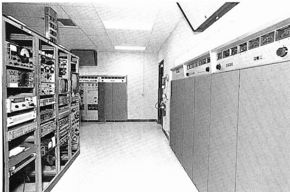
WMVS/WMVT share transmitting space, with their TT-35FH, 35 kW VHF transmitter and TTU-60D, 60 kW UHF transmitters also sharing monitoring and control facilities.
