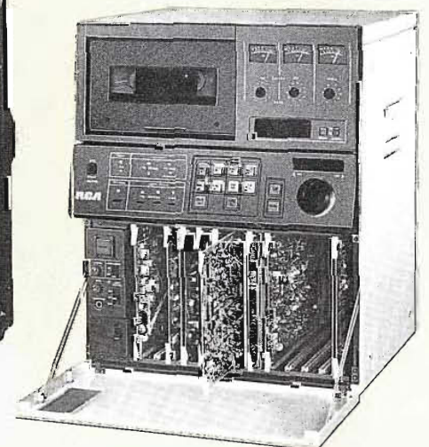
HR-2 Studio VTR, with lower panel dropped, showing front access to plug-in modules.
