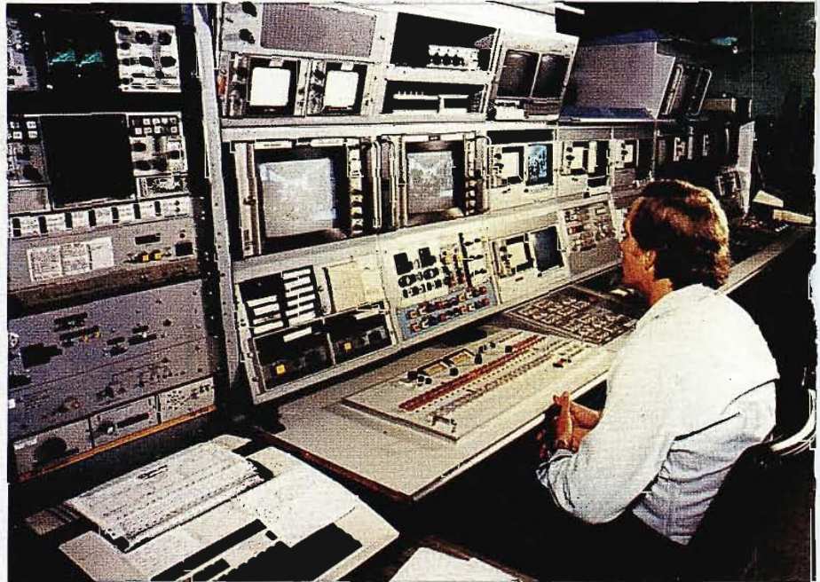
Master Control is an integral part of KCPQ's Technical Center. Machine controls and live and film camera video controls are built into the MC console.
